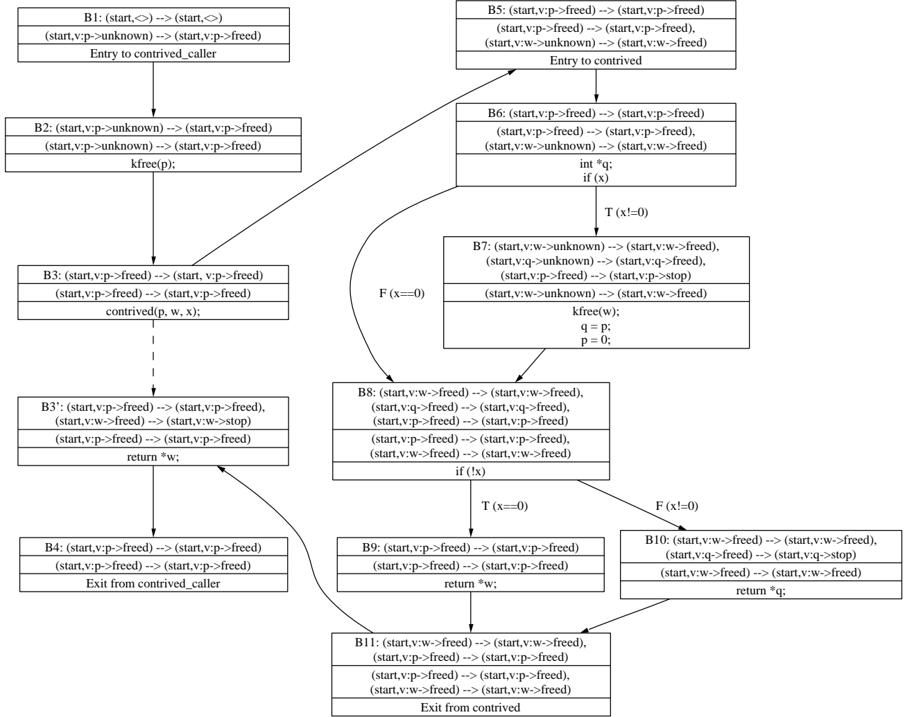
Figure 5: Supergraph for the example code shown in Figure 2. The top field in each basic block shows the block summary, the middle field shows the suffix summary, and the bottom field shows the source code in the block. Each block's number is listed in the first field. Note that none of the suffix summaries record any information about q because q is a local variable so the analysis would never use these edges. Edges that start and end in a tuple containing the placeholder \langle \rangle are omitted from the cache unless this tuple is the only element in the cache. Also, the suffix summary intentionally omits edges that end in a tuple with the value stop . Suffix edges are only relaxed along traversed paths, i.e. those not suppressed by the algorithm described in Section 8. The analysis does not follow calls to kfree because the extension matches these calls. Thus, they are not considered callsites in the supergraph construction.
