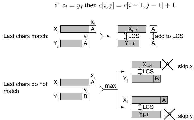
Fig. 5: The possible cases in the DP formulation of LCS.
