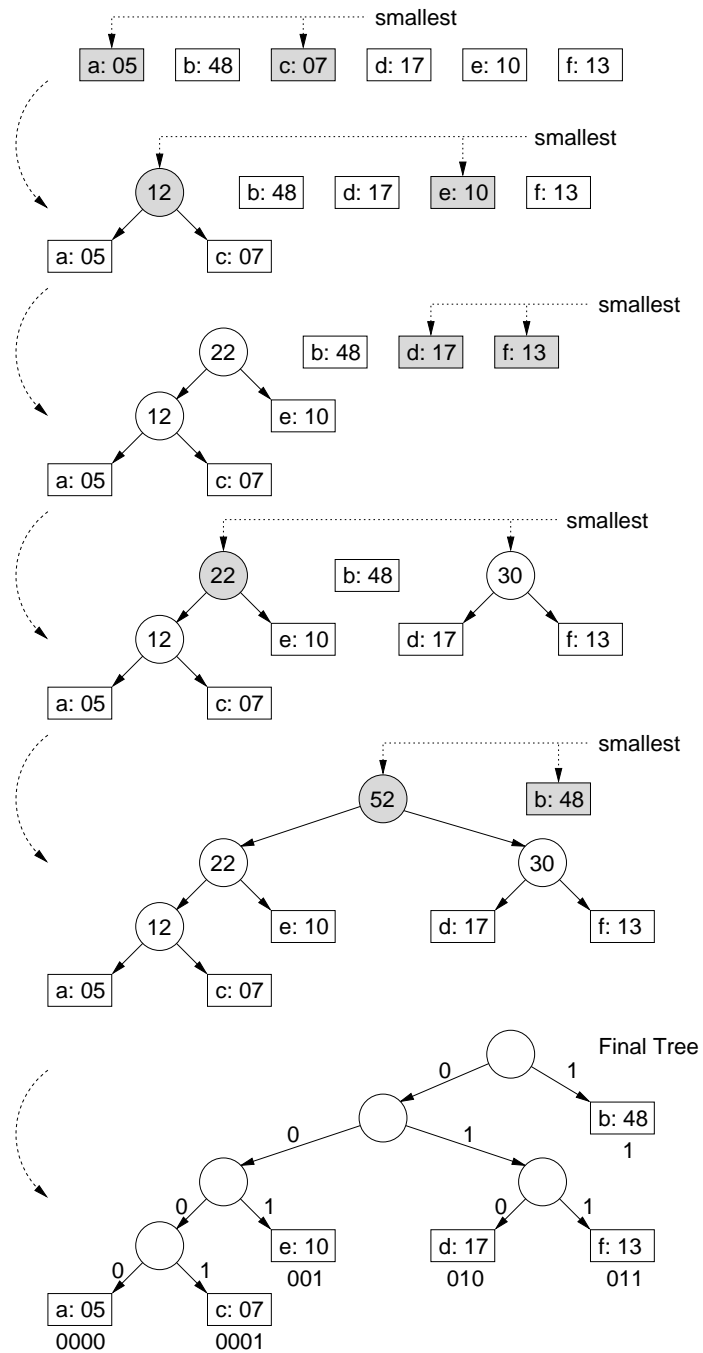
Fig. 18: Huffman's Algorithm.
