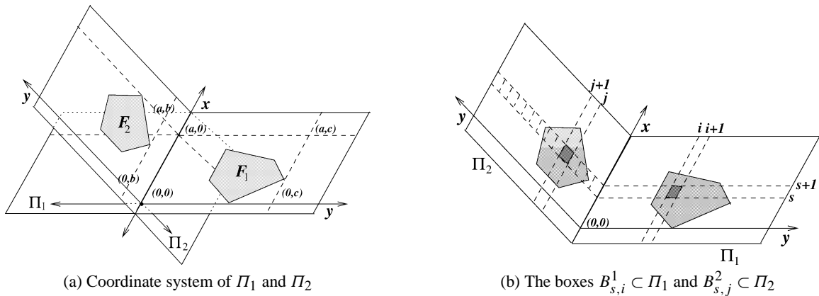
Fig. 8. The case that \Pi_1 \not\parallel \Pi_2 .
