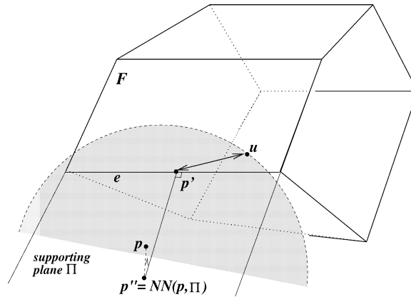
Fig. 12. Good Type-III sphere S with p outside \mathcal{P} . In this case no matter how large the radius of S is, the area of the intersection of S with \mathcal{P} can be arbitrarily small. This means that even if S is a good sphere, it is quite possible that the points in S \cap F are very far away from p'' , the center of the disk B = S \cap \Pi . For example, in this figure, we are not able to bound d(p', u) for u \in B \cap F .
