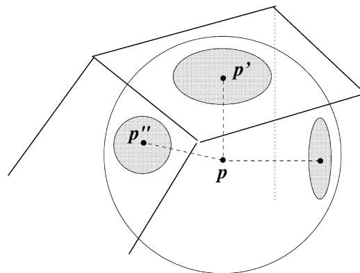
Fig. 4. An example of a Type-II sphere. p , the center of the sphere, is inside polytope \mathcal{P} (for clarity many of the faces of \mathcal{P} have been left out of the diagram). For all the faces F_i of \mathcal{P} that the sphere intersects, the center of the intersection disk with the supporting plane \Pi_i is on F_i .
