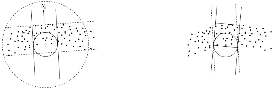
Fig. 3. On the left, the initial candidate neighborhood is the one perpendicular to strip(s) . On the right, as we rotate the candidate neighborhood, we maintain the smallest bounding rectangle of all samples inside.
