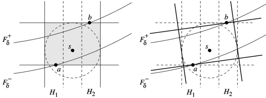
Fig. 13. In the right figure, the middle bold rectangle is the one obtained by a slight anti-clockwise rotation. Its height is smaller than that of the middle dashed rectangle.
