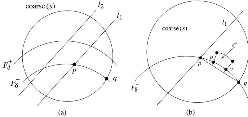
Fig. 9. (a) Illustrates that F_\delta^-(p, q) lies below l_1 ; (b) illustrates our choice of a cell C that lies below l_1 .
