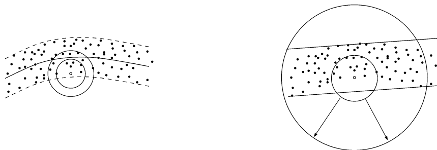
Fig. 2. On the left, the white dot is the sample s , the inner disk is D , and the outer disk is initial(s) . On the right, we grow initial(s) until strip(s) has a relatively large aspect ratio. The final disk is coarse(s) .
