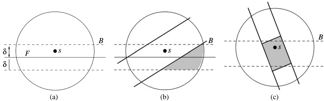
Fig. 4. The left figure shows coarse(s) , the noise band B , and F . In the middle figure, the bold strip is strip(s) and the shaded area is the significant area of B outside strip(s) . The shaded area should be non-empty with high probability. In the right figure, the shaded rectangle is the candidate rectangle.
