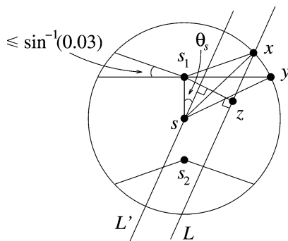
Fig. A.4. Illustration for Lemma 8.1(iii).
