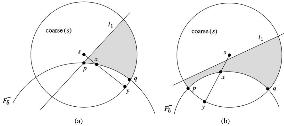
Fig. 10. The shaded region denotes \mathcal{R} in both figures. In (a), q is the closest point in R to x . In (b), p or q is the closet point in R to x .
