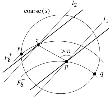
Fig. 11. Rotating \ell_1 and \ell_2 slightly in the clockwise direction decreases the width of strip(s) .
