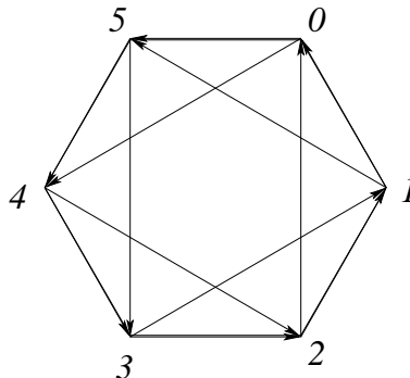
Figure 1: The directed circulant graph \vec{C}_6^{4,5} .
