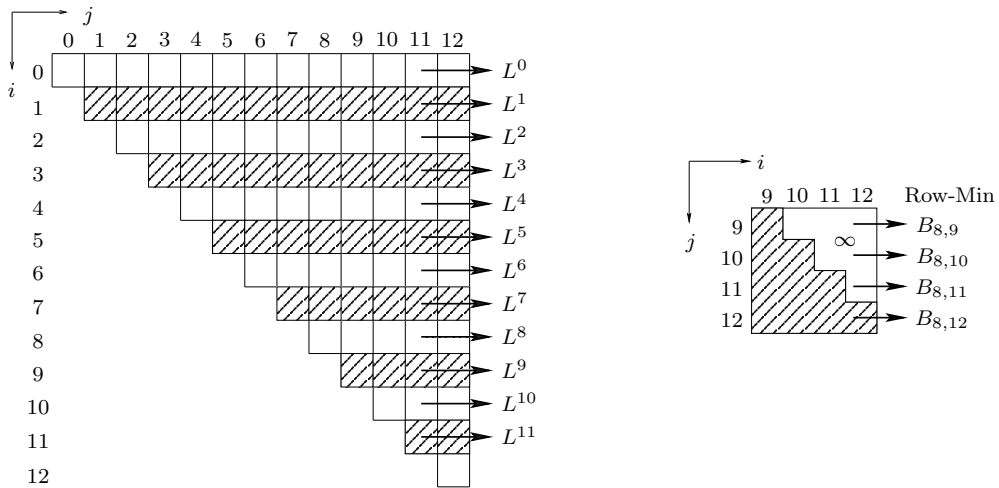
Figure 5: The left-hand figure shows the B_{i,j} matrix for n = 12 . Each row in the B_{i,j} matrix will correspond to a totally monotone matrix L^m . The minimal element of row j in L^m will be the value B_{m,j} . The righthand figure shows L^8 .
