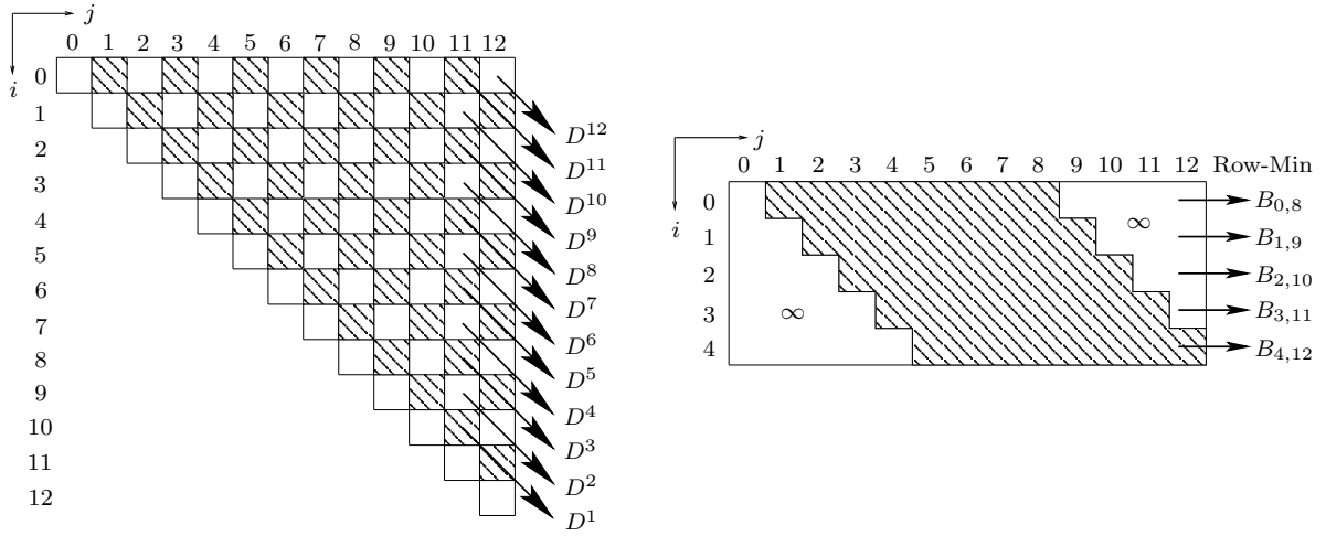
Figure 3: The left-hand figure shows the B_{i,j} matrix for n = 12 . Each diagonal, d = i - j , in the matrix will correspond to a totally monotone matrix D^d . The minimal item of row i in D^d will be the value B_{i,i+d} . The righthand figure shows D^8 .
