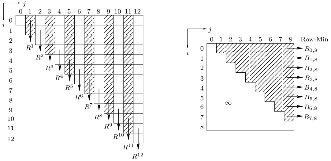
Figure 4: The left-hand figure shows the B_{i,j} matrix for n = 12 . Each column in the B_{i,j} matrix will correspond to a totally monotone matrix R^m . The minimal element of row i in R^m will be the value B_{i,m} . The righthand figure shows R^8 .
