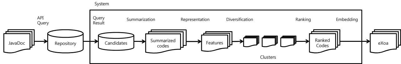
Figure 3: Process of Automatic Example Oriented API Document Generation
