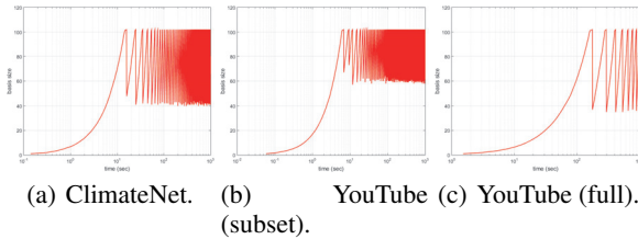
Figure 3: Basis size obtained by FFWTensor.
