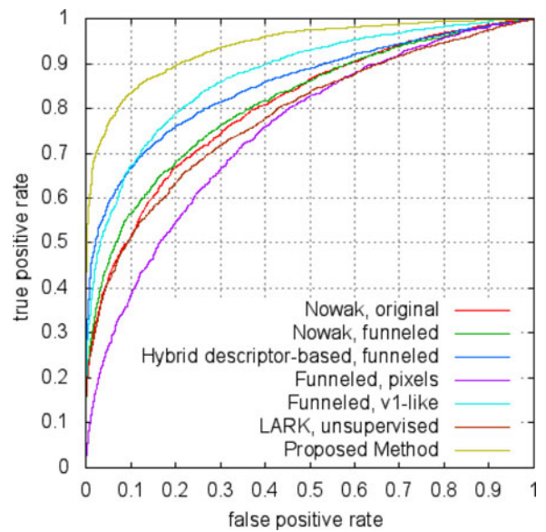
Fig. 12. The ROC curve comparisons between the proposed method and other state-of-the-art methods on the LFW database.
