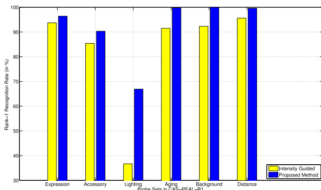
Fig. 9. Rank-1 recognition rates of the six probe sets on the CAS-PEAL-R1 database by using the proposed method and using pixel intensity guided registration strategy.
