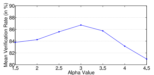
Fig. 13. The mean face verification rates with different values of \alpha in Equation (4) on the LFW database.
