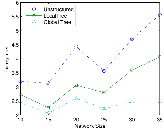
Fig. 3: Energy cost vs. network size.
