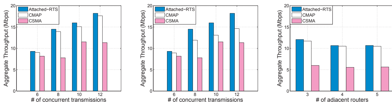
Fig. 17: Aggregate throughput in static ad hoc networks with different # of concurrent transmissions Fig. 18: Aggregate throughput in mobile ad hoc networks with different # of concurrent transmissions Fig. 19: Aggregate throughput in mesh networks with different # of adjacent routers, each with 3 clients
