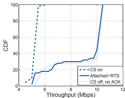
Fig. 14: Aggregate throughput of Exposed Terminal Configuration
