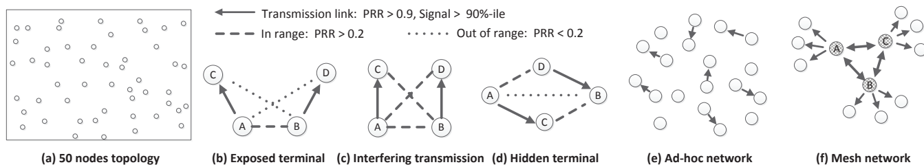
Fig. 13: Topologies overview, with 50 nodes basic test bed(a), base line topology (b) (c) (d) in Sec. 4.2.1, and practical networks (e) (f) in Sec. 4.2.2. Link constraints are included in the figure.
