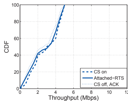
Fig. 16: Aggregate throughput of Hidden Terminal Configuration
