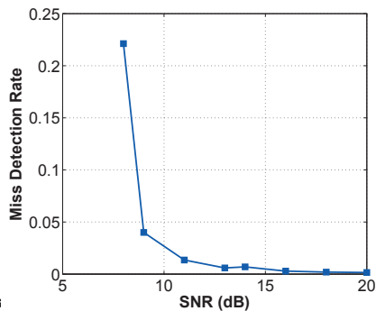
Fig. 10: Decodability of Data Transmission with/without Attachment Transmission under different SNRs Fig. 11: Impact of number of concurrent Attachment Transmission under different SNRs Fig. 12: Miss detection rate under different SNRs
