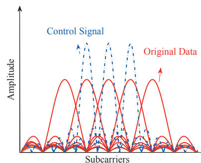
Fig. 2: An illustration of Attachment Coding to transmit control messages and data packets together
