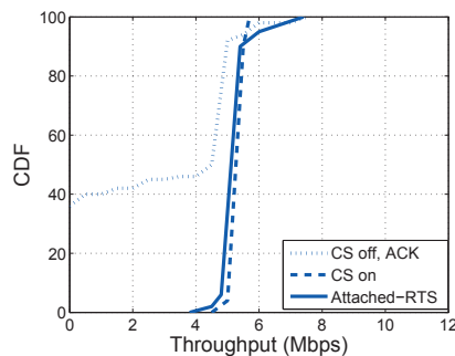
Fig. 15: Aggregate throughput of Interfering Terminal Configuration
