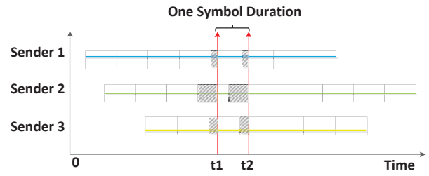
Fig. 6: Cyclic Attached RTS
