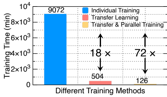
Figure 20. Training speedup techniques
