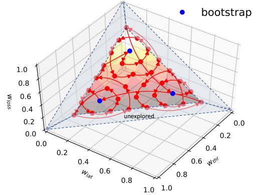
Figure 4. The objective training trajectory for fast traversing, generated by neighbourhood-based objective sorting algorithm (details in §4.2).
