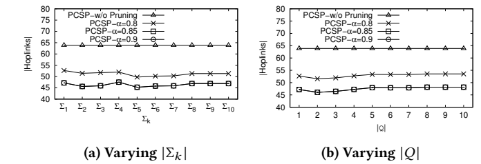
Figure 10: Ablation study on NY
