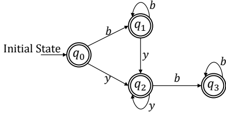
Figure 2: A DFA for b^*y^*b^*
