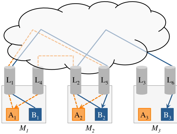
Figure 3: Two VMs from tenant-A (orange) and three from tenant-B (dark blue) and their communication patterns over a 3 \times 3 datacenter fabric. The network fabric has three uplinks ( L_1 - L_3 ) and three downlinks ( L_4 - L_6 ) corresponding to the three physical machines.
